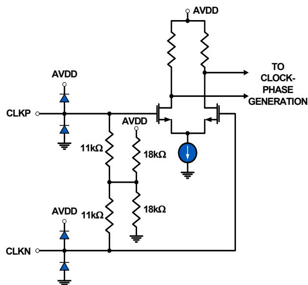
FIGURE 43. CLOCK INPUTS
