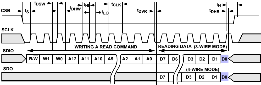
SPI READ FIGURE 37. SPI READ
