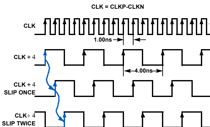
FIGURE 40. PHASE SLIP: CLK ÷ 4 MODE, f_{\text{CLK}} = 1000\text{MHz}
