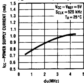
Power Supply Current vs \phi_2 Clock Frequency
