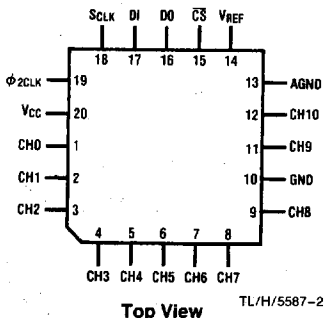
Molded Chip Carrier (PCC) Package
