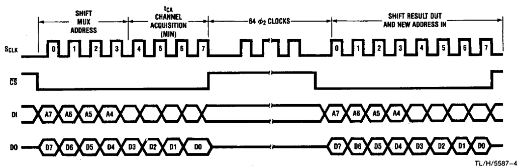
\overline{CS} High During Conversion
