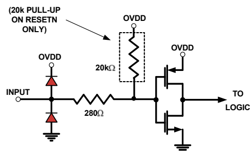
FIGURE 51. DIGITAL INPUTS
