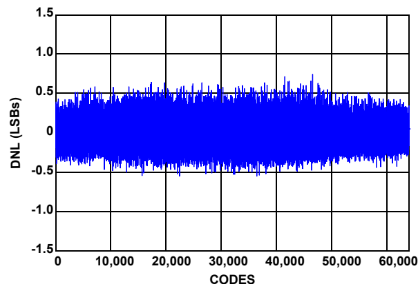
FIGURE 9. DIFFERENTIAL NONLINEARITY
