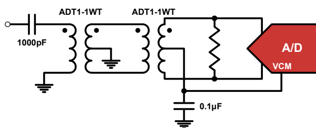
FIGURE 27. TRANSFORMER INPUT FOR GENERAL PURPOSE APPLICATIONS
