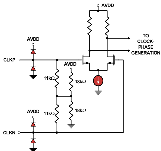
FIGURE 48. CLOCK INPUTS
