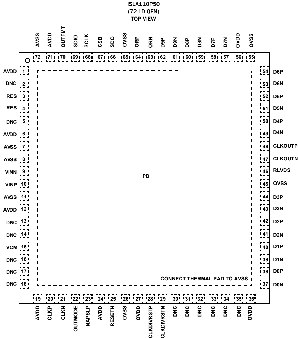
FIGURE 2. PIN CONFIGURATION
