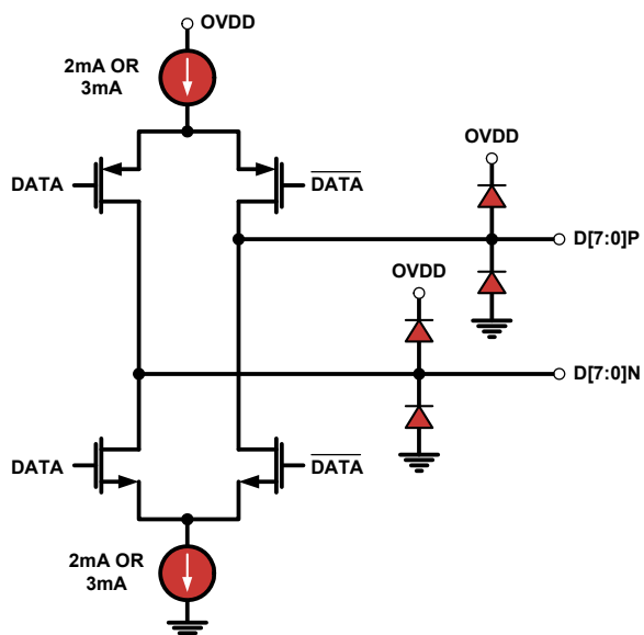
FIGURE 51. LVDS OUTPUTS
