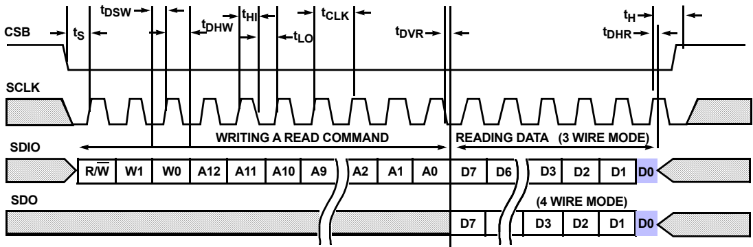
SPI READ
