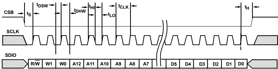
SPI WRITE
