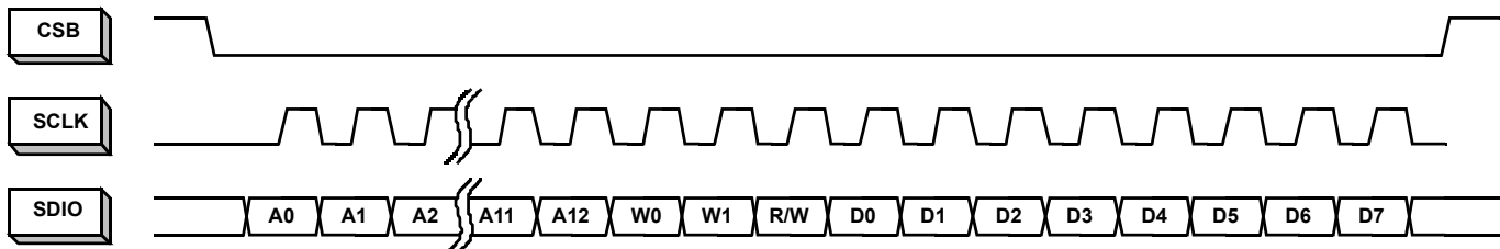
FIGURE 40. LSB-FIRST ADDRESSING
