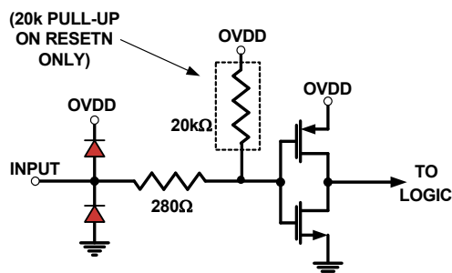
FIGURE 50. DIGITAL INPUTS
