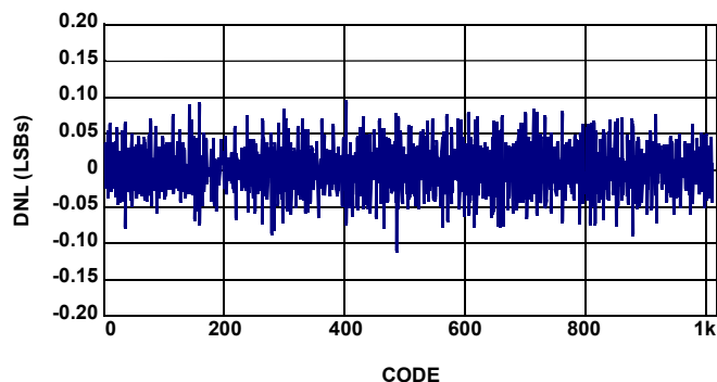
FIGURE 12. DIFFERENTIAL NONLINEARITY
