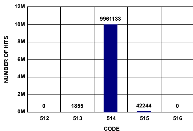
FIGURE 15. NOISE HISTOGRAM
