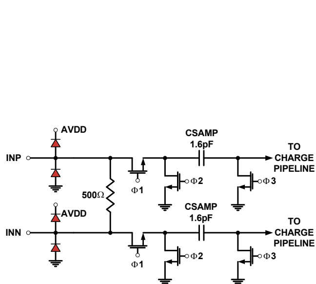
FIGURE 47. ANALOG INPUTS
