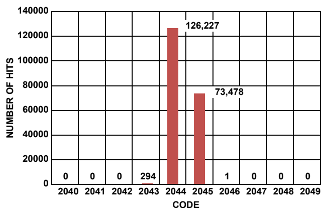
FIGURE 13. NOISE HISTOGRAM
