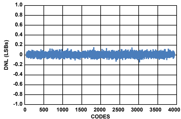
FIGURE 10. DIFFERENTIAL NONLINEARITY
