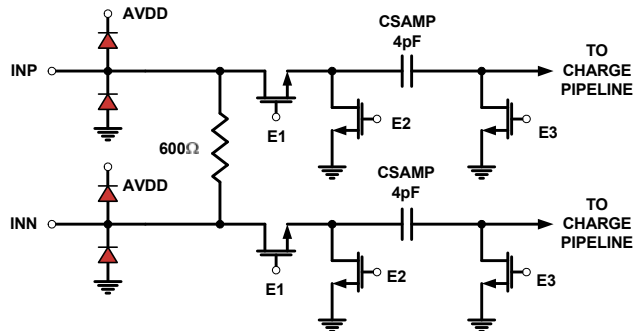
FIGURE 43. ANALOG INPUTS
