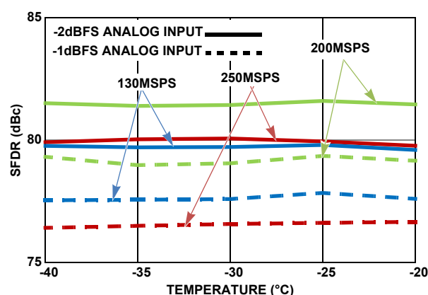
FIGURE 22. TYPICAL SFDR PERFORMANCE vs TEMPERATURE, DEVICE CALIBRATED AT -40°C, f_{IN} = 105\text{MHz}
