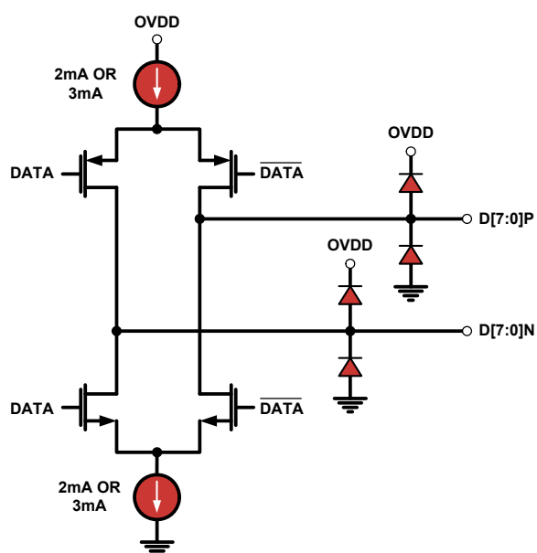
FIGURE 51. LVDS OUTPUTS
