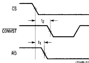
Figure 15. CS to CONVST Setup Timing
