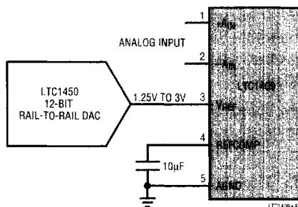
Figure 9. Driving V_{\text{REF}} with a DAC
