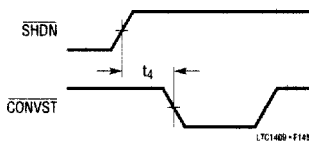
Figure 14b. SHDN to CONVST Wake-Up Timing
