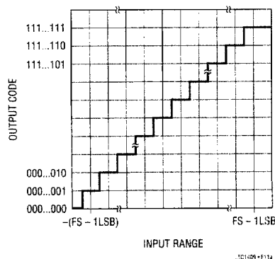
Figure 11a. LTC1409 Transfer Characteristics
