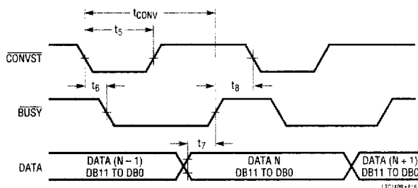
Figure 16. Mode 1a. \text{CONVST} Starts a Conversion. Data Outputs Always Enabled ( \text{CONVST} = \square )
