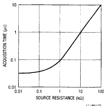
Figure 6. Acquisition Time vs Source Resistance
