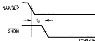
Figure 14a. NAP/SLP to SHDN Timing
