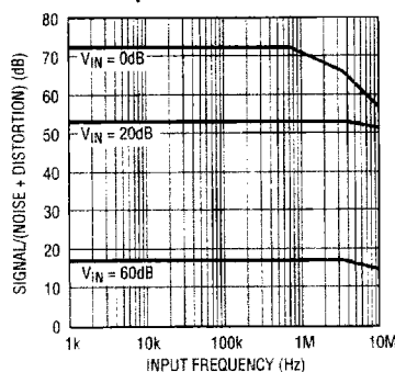
S/(N + D) vs Input Frequency and Amplitude
