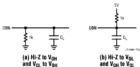
Load Circuits for Access Timing
