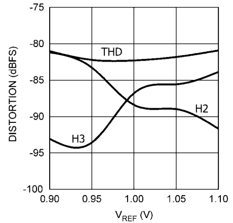
DISTORTION vs. V_{REF}
