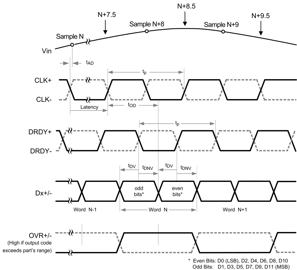
Output Timing
