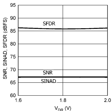
SNR, SINAD, SFDR vs. V_{DR}
