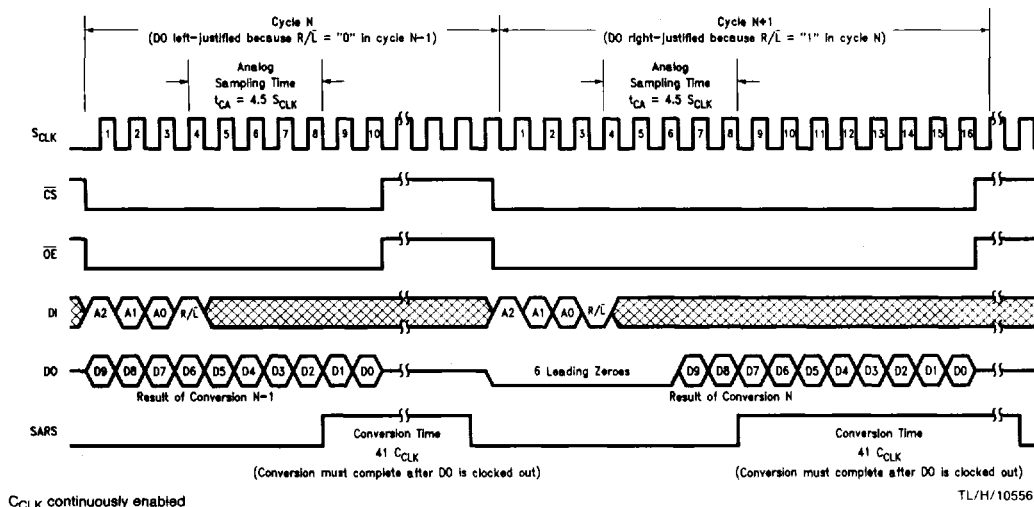
ADC1038/ADC1034 \overline{CS} High during Conversion
