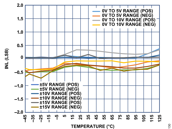
Figure 27. INL vs. Temperature
