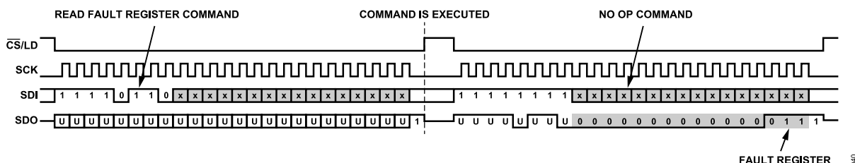
Figure 45. Typical Read Command Sequence for 24-Bit Words
