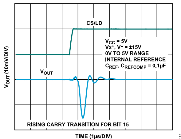
Figure 15. Glitch Impulse
