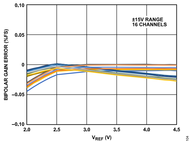
Figure 4. Gain Error vs. V_{REF}
