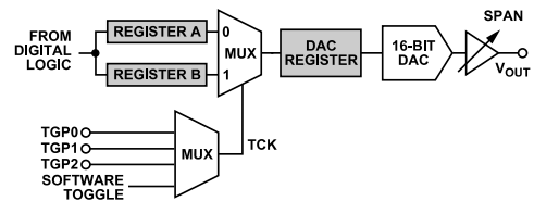
Figure 47. Toggle Operation
