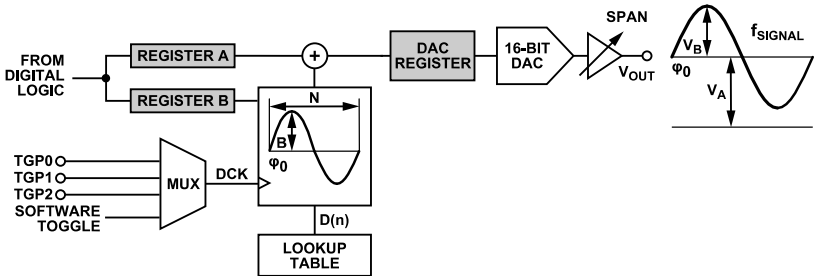
Figure 49. Dither Signal Operation
