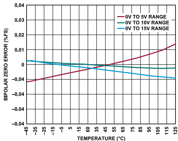
Figure 30. Bipolar Zero Error vs. Temperature
