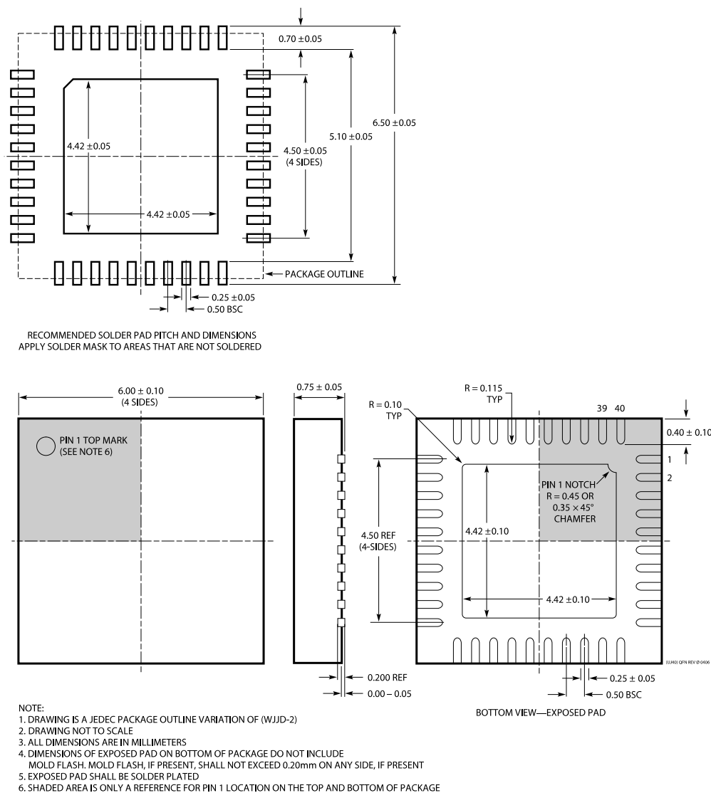
Figure 55. 40-Lead Lead Frame Chip Scale Package [LFCSP] 6 mm × 6 mm Body and 0.75 mm Package Height 05-08-1728 Dimensions shown in millimeters
