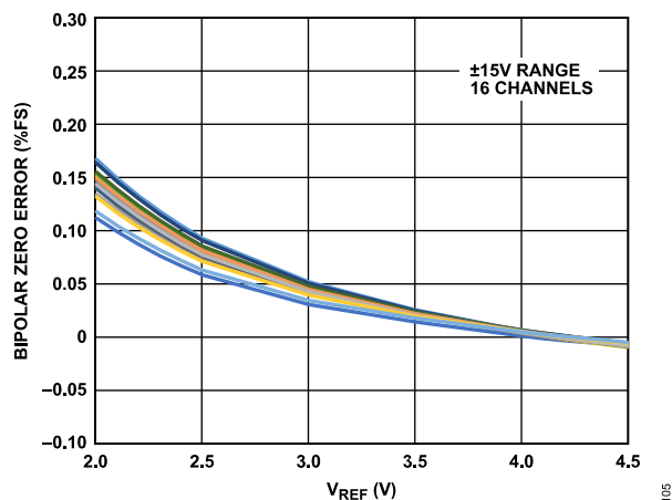
Figure 5. Bipolar Zero Error vs. V_{REF}
