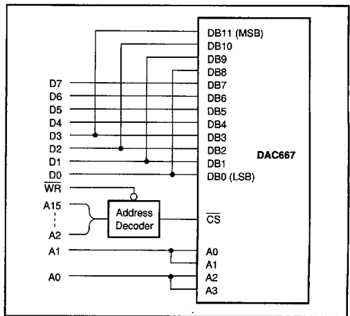
FIGURE 11. Right-Justified 8-Bit Bus Interface.
