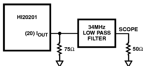
FIGURE 6. HI20201 GLITCH TEST CIRCUIT
