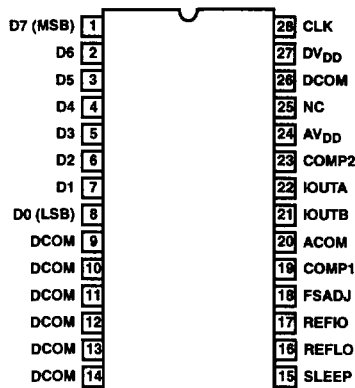
HI5660 (SOIC, TSSOP) TOP VIEW
