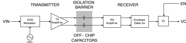
Figure 13. Operational Block Diagram of Single Channel
