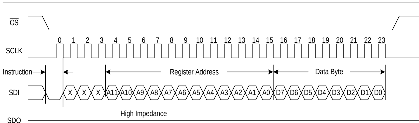
Figure-22 Write Operation In SPI Mode
