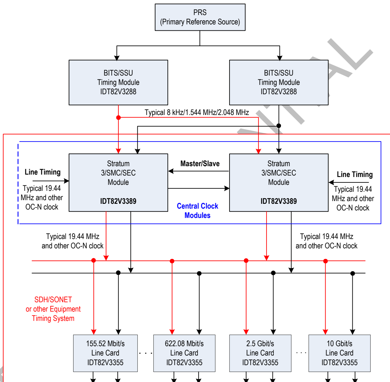
Figure 17. Typical Application
