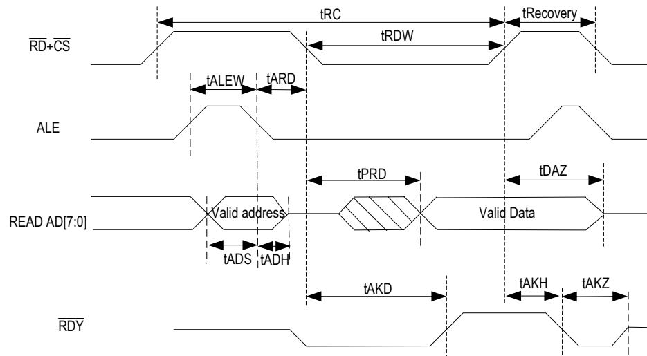
Figure-31 Multiplexed Intel Read Timing
