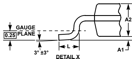
DETAIL X
