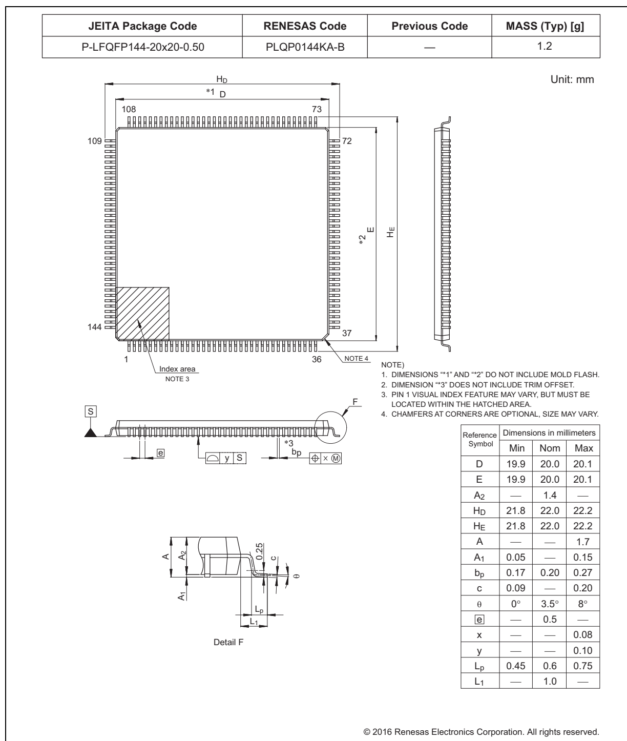
Figure 1.2 144-pin LQFP
