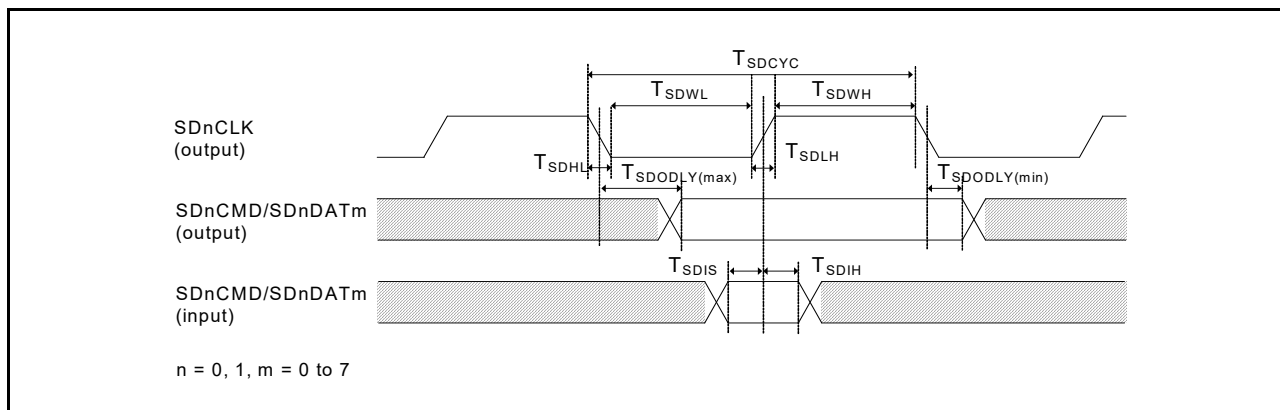
Figure 2.63 SD/MMC Host Interface signal timing
