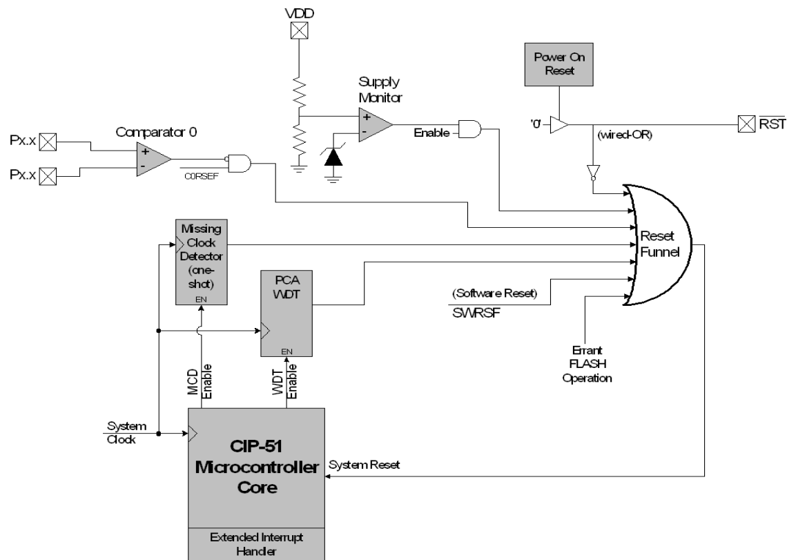
Figure 21.1. Reset Sources
