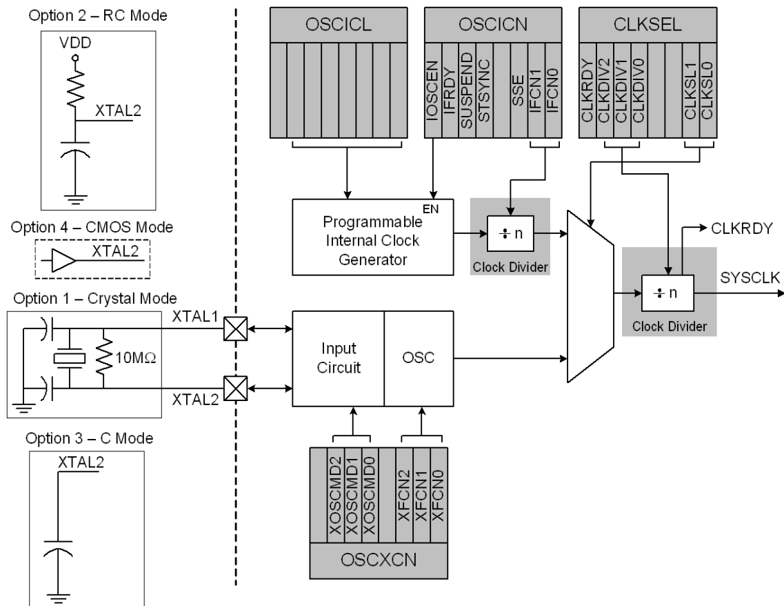
Figure 22.1. Oscillator Options
