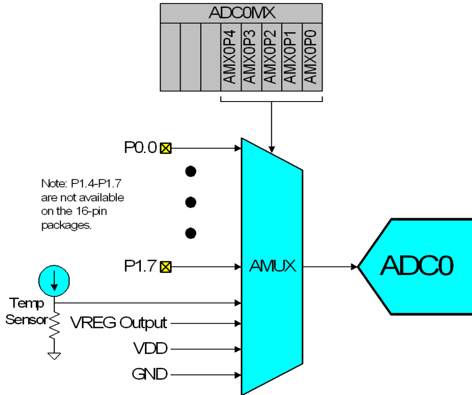
Figure 8.6. ADC0 Multiplexer Block Diagram
