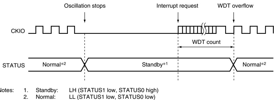
Figure 22.4 Software Standby to Interrupt STATUS Output
