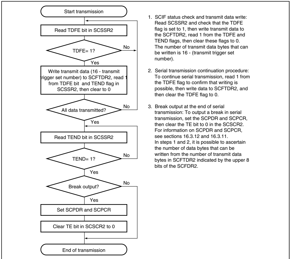
Figure 16.6 Sample Serial Transmission Flowchart
