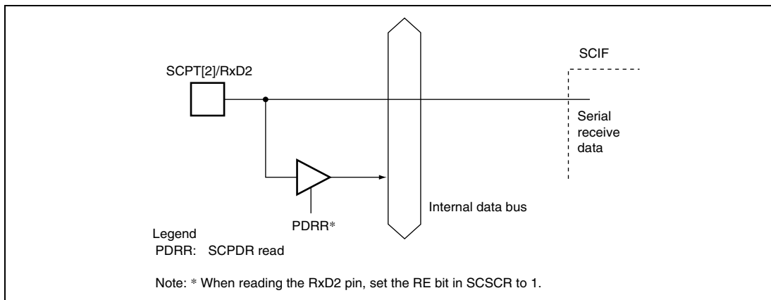
Figure 16.4 SCPT[2]/Rx2 Pin
