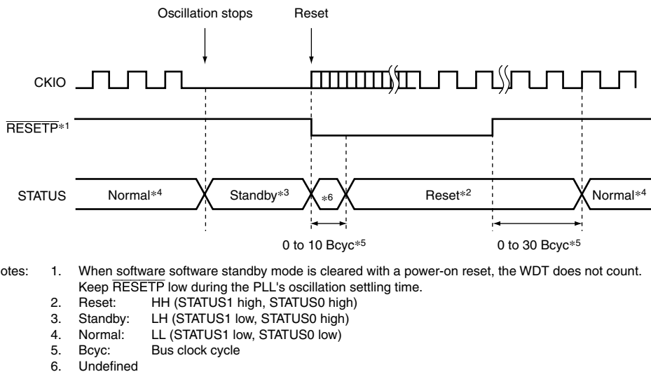
Figure 22.5 Software Standby to Power-On Reset STATUS Output
