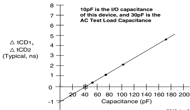
Figure 3. Typical Output Derating (Lumped Capacitive Load).
