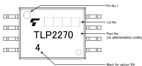
Fig. 16.4 Marking Example (Note)
