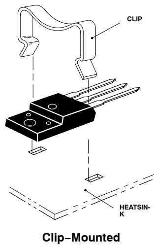
Figure 4. Typical Mounting Technique
