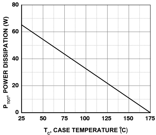
Figure 5. Power Derating
