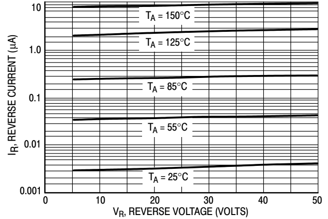
Figure 3. Leakage Current
