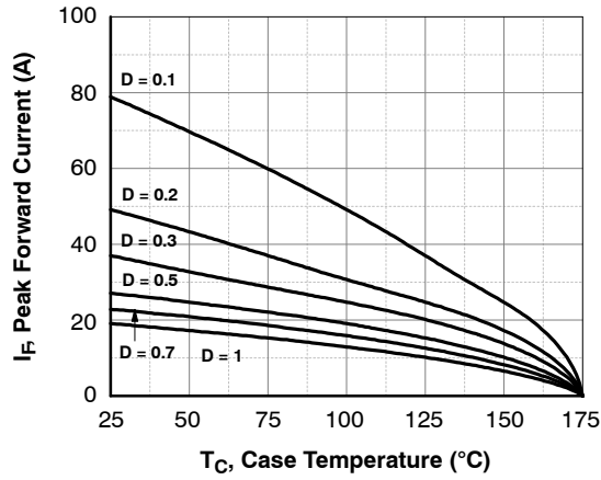
Figure 3. Current Derating
