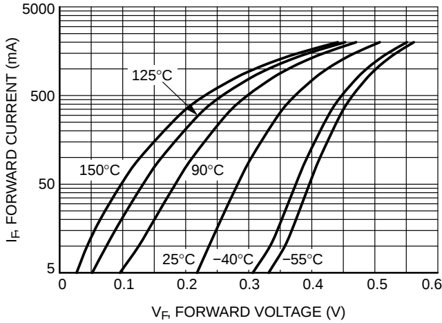
Figure 5. Forward Voltage
