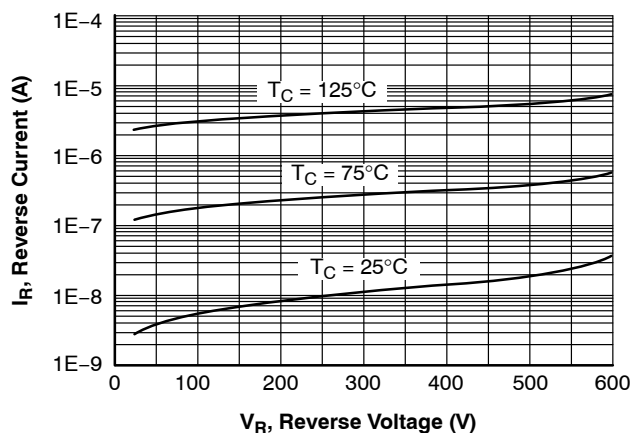
Figure 6. Typical Reverse Current
