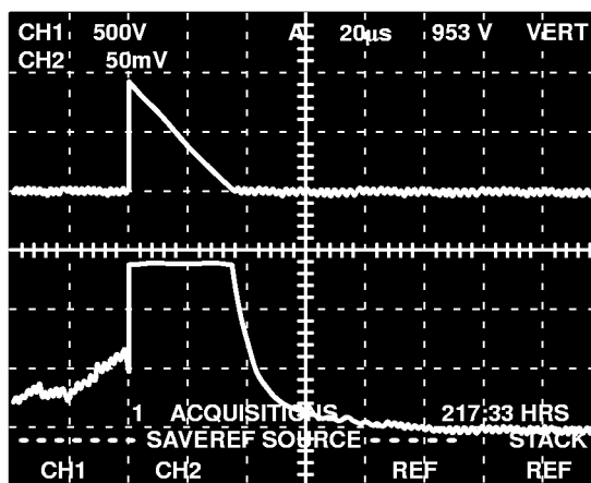
Figure 11. Current–Voltage Waveforms
