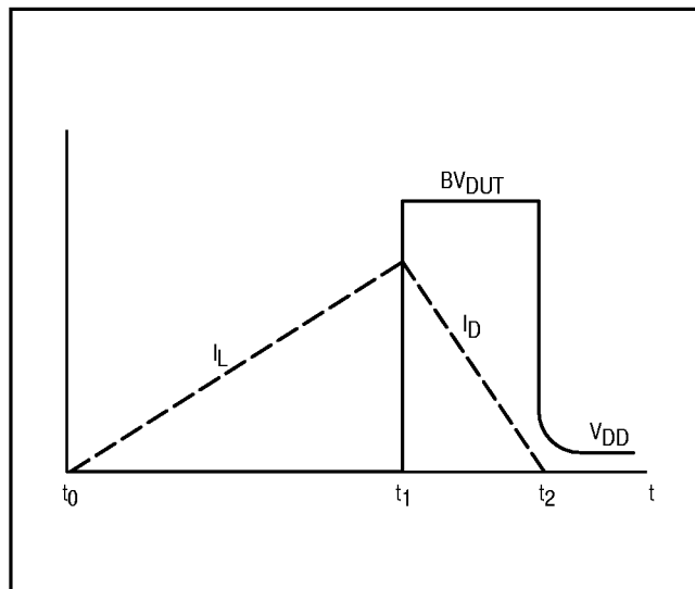
Figure 10. Current–Voltage Waveforms
