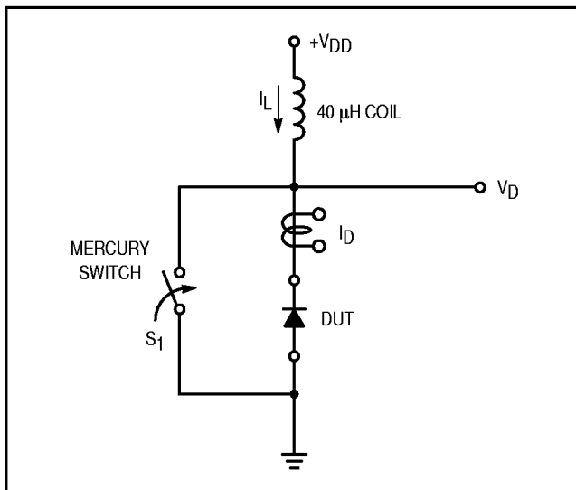
Figure 9. Test Circuit
