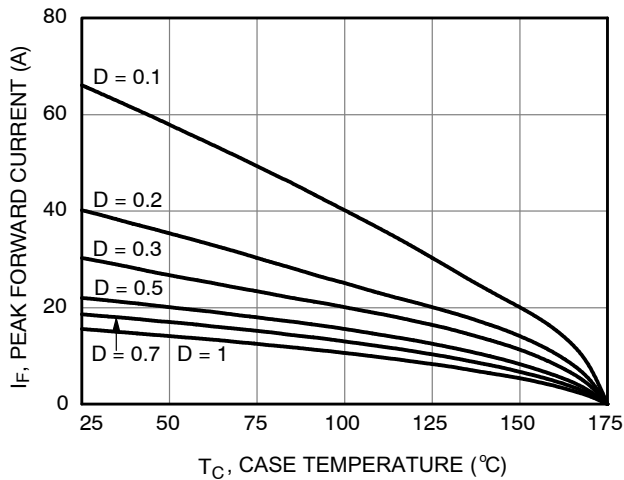
Figure 3. Current Derating
