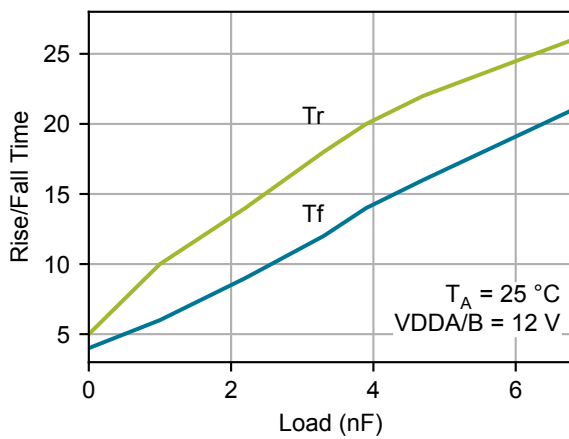
Figure 4.5. Rise/Fall Time vs. Load
