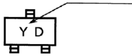
Fig. 9.4 Marking RN2104
