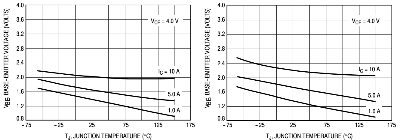
Figure 5. Base-Emitter Voltage
