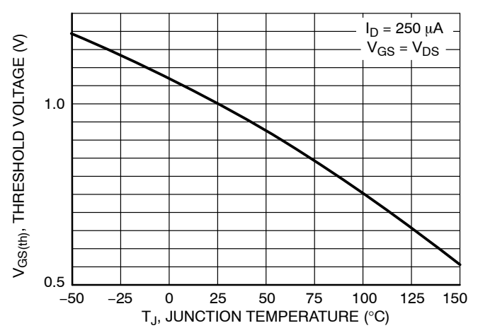
Figure 11. Threshold Voltage
