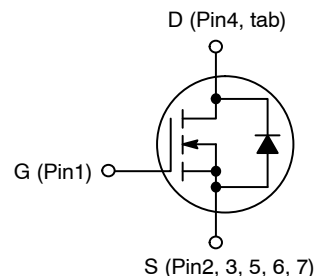
N-Channel MOSFET
