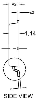
LFPK8 5x6 CASE 760AA ISSUE C
