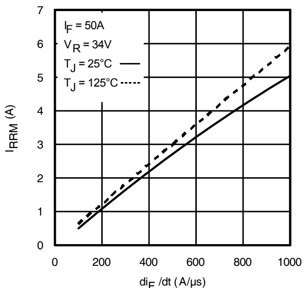
Fig. 20 - Typical Recovery Current vs. di/dt
