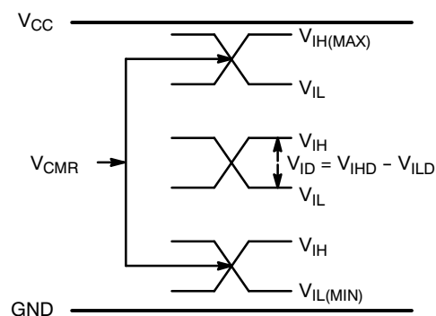
Figure 8. V_{CMR} Diagram
