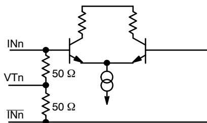
Figure 4. Input Structure
