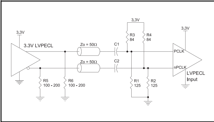
Figure 2B. PCLK/nPCLK Input Driven by a 3.3V LVPECL Driver with AC Couple
