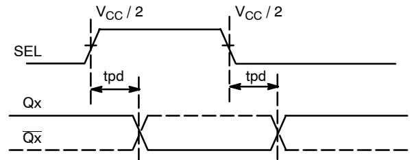
Figure 9. SEL to Qx Timing Diagram
