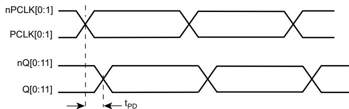
Figure 9. Propagation Delay
