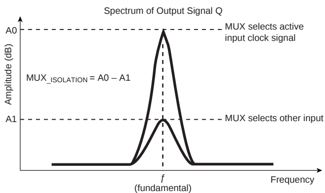
Figure 10. MUX Isolation
