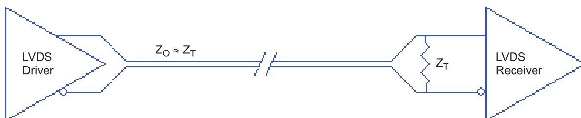
Figure 9. Optional LVDS Termination
