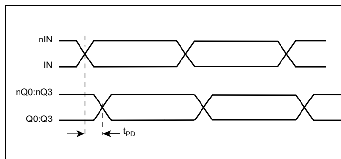
Propagation Delay
