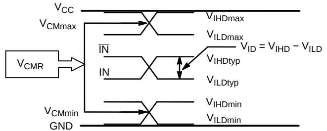
Figure 10. V_{CM} Diagram
