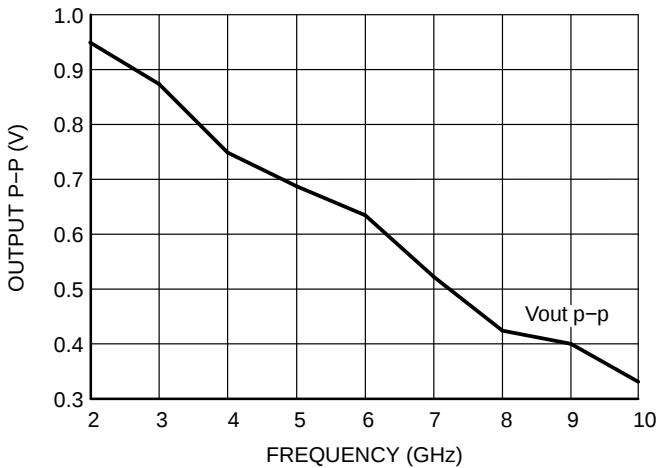
Figure 2. Typical V_{\text{OUT P-P}} vs. Frequency at 25^{\circ}\text{C}
