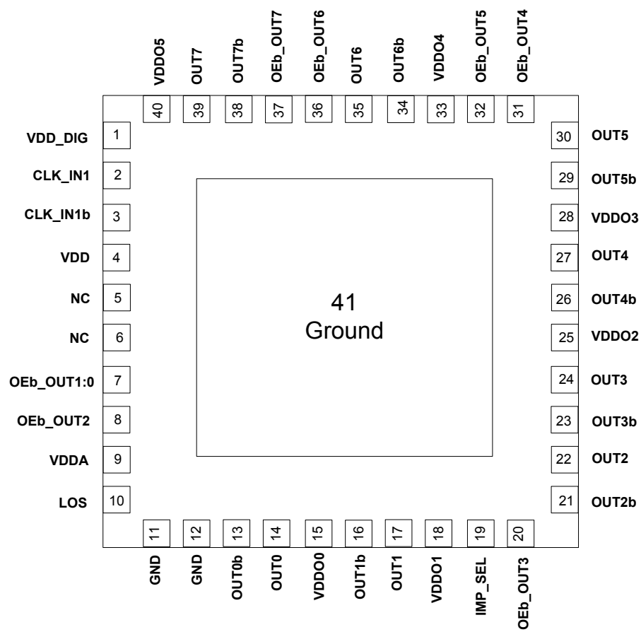
Figure 6.1. Si53258A-D01AM 40-QFN
