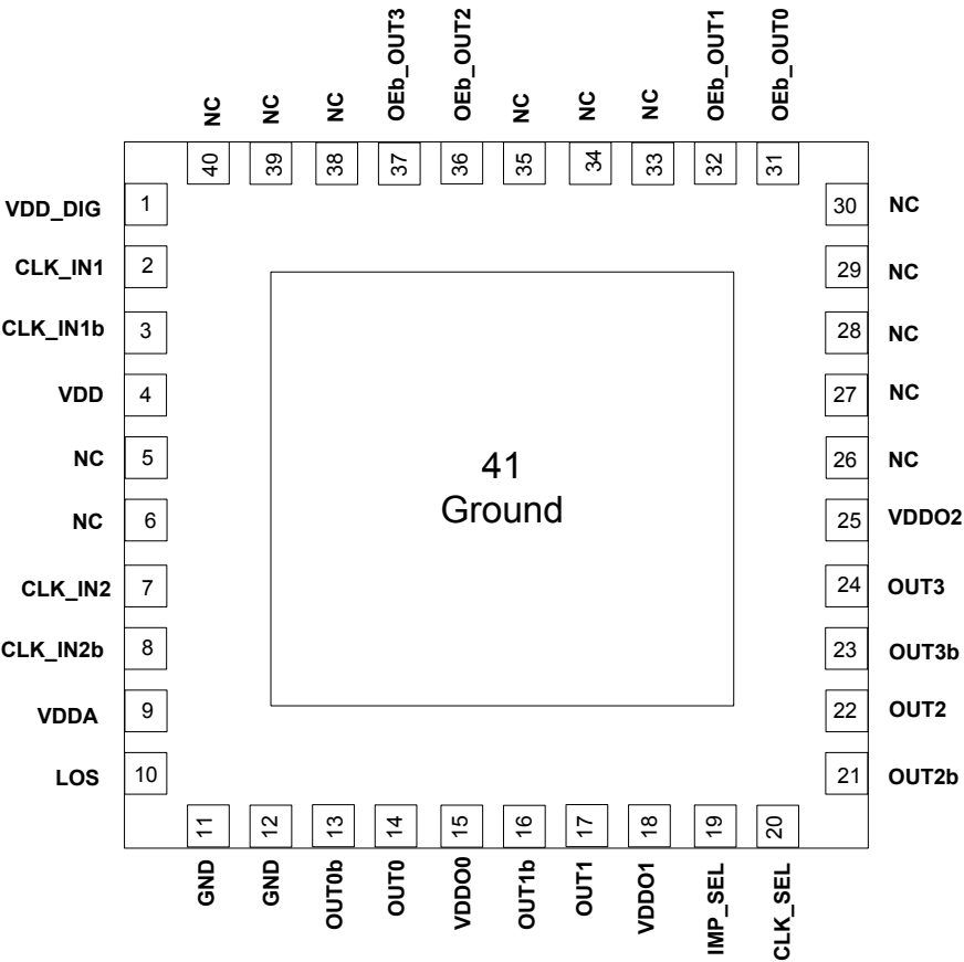
Figure 6.4. Si53254A-D02AM 40-QFN
