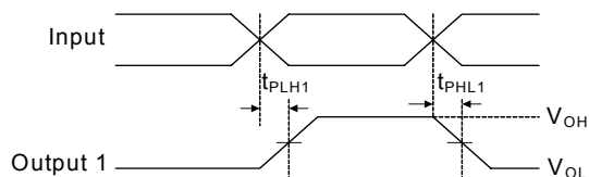
Figure 4. Pulse Skew ( t_{SK(p)} = |t_{PLH} - t_{PH}| )
