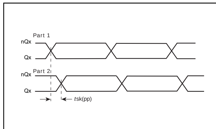
Part-to-Part Skew
