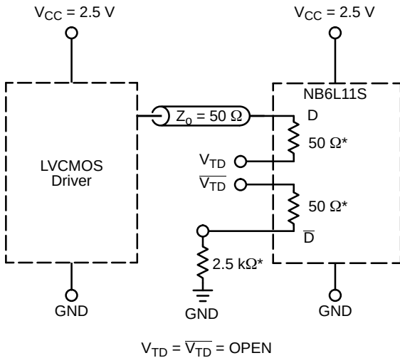
Figure 15. LVCMOS Interface
