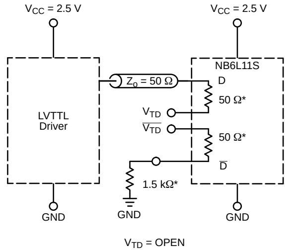
Figure 16. LVTTTL Interface
